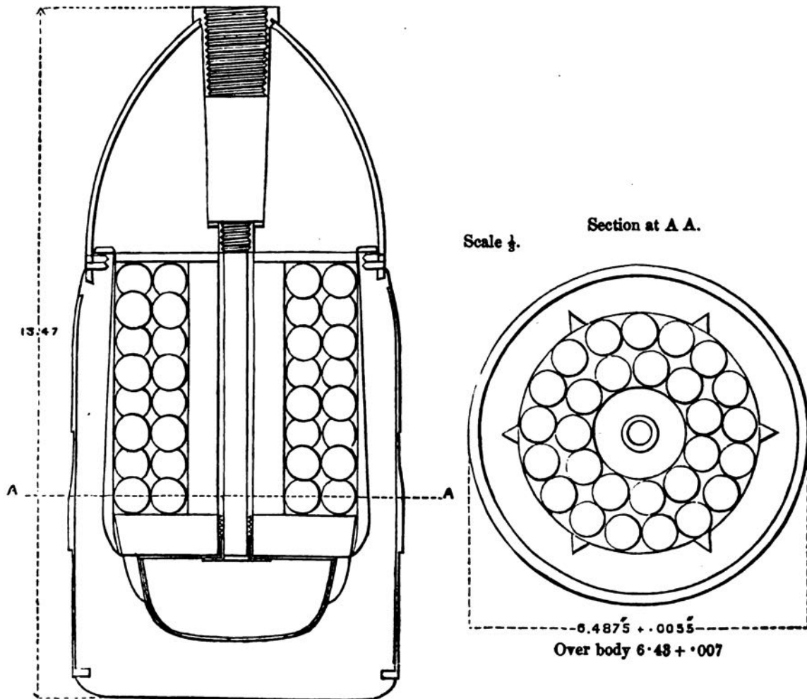
Boxer Shrapnel 64-PR. B.L. II.
