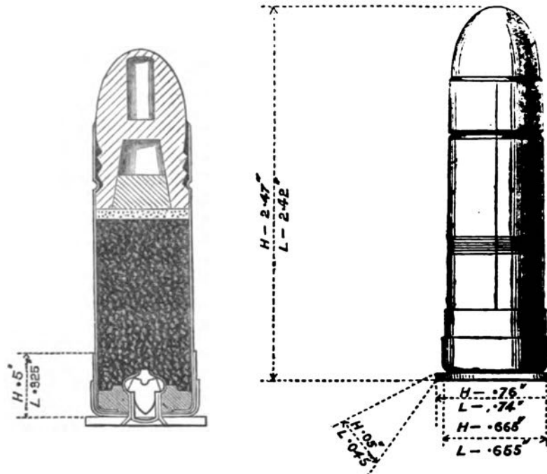
Cartridge, Mark IX., Snider arm.
