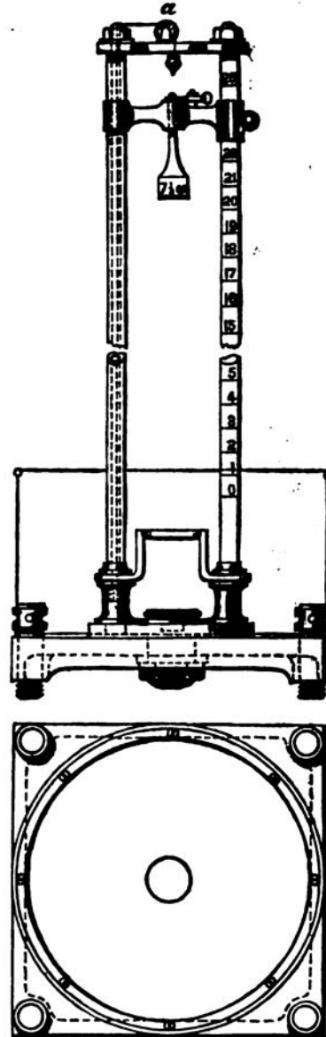
Stand for proving detonators of Pettman fuzes, and of B.L. time fuzes.
