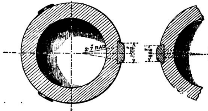
80-PR. COMMON SHELL. MARK L.
