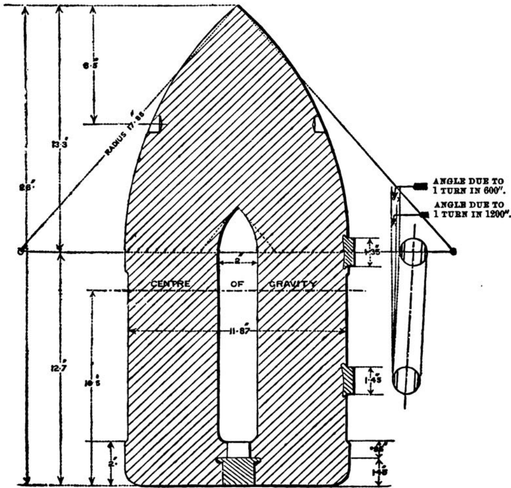
PALLISER SHOT, 12", I. (Base closed by a plug hammered in.)
