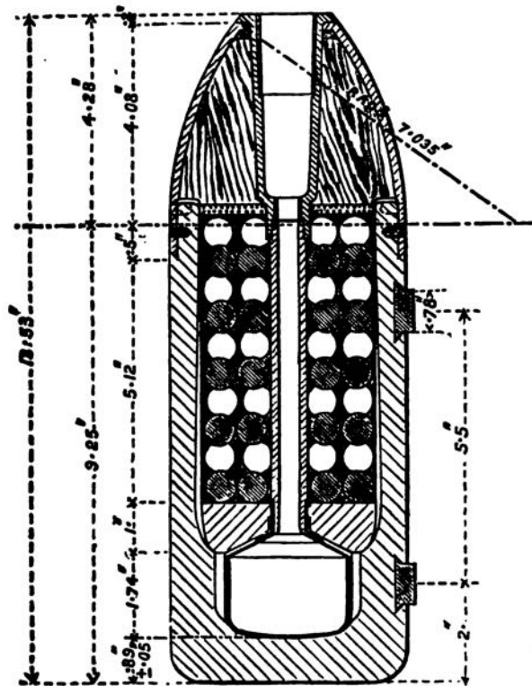
40-PR. SHRAPNEL SHELL. MARK I.
